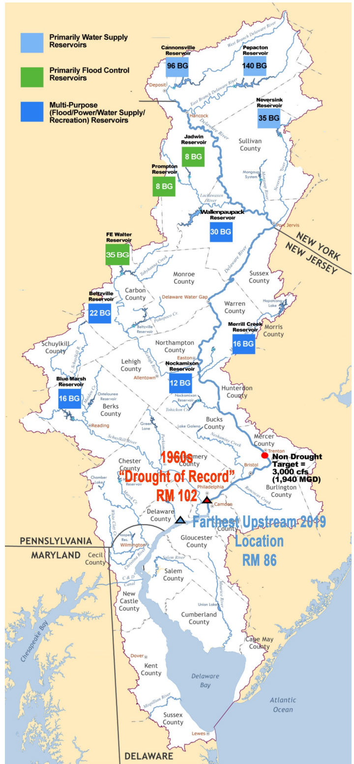
Reservoirs in the Basin have many purposes, including: water supply, hydropower generation, recreation and flood control. BG = Billion Gallons. MGD = Million Gallons/Day.
