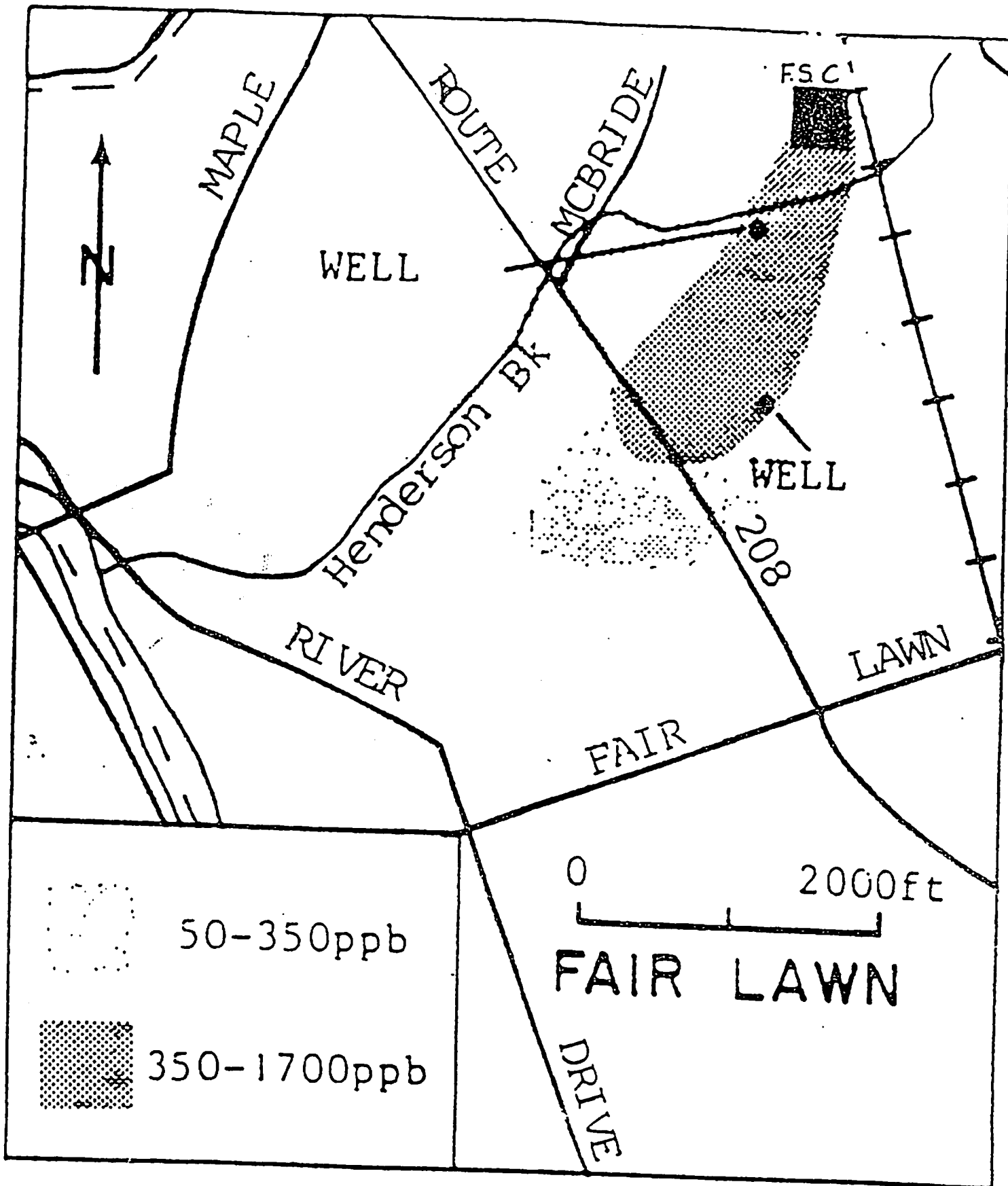
Fig. 4. contaminant plume. Carbon tetrachloride and chloroform concentrations (1982-1983).
