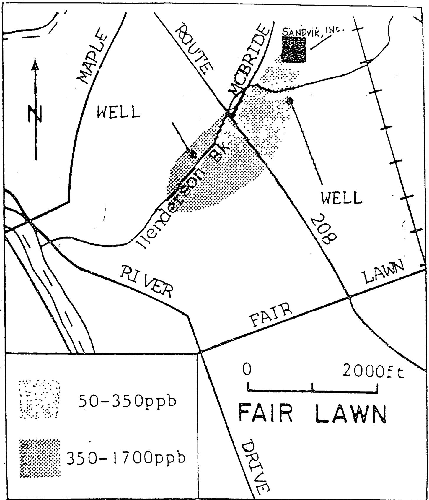
Fig. 3. contaminant plume. 1,1,1-trichloroethane, and tetrachloroethylene concentrations (1982-1992)
