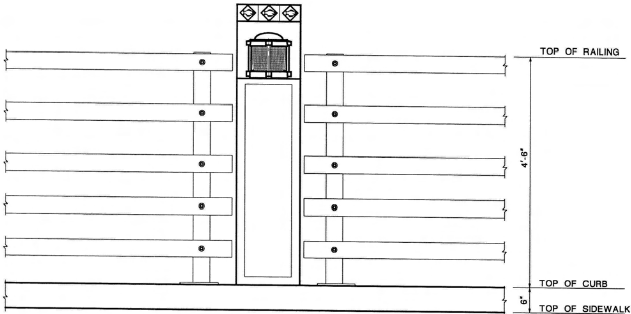
ROUTE 36 PEDESTRIAN BRIDGE LIGHTING LIGHTING SHOWN ON RAMP SPANS
