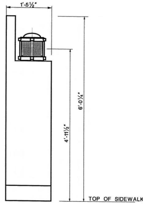
SECTION
